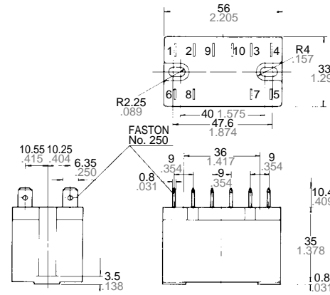
2 coil latching
