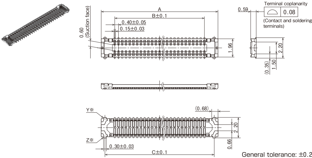
Dimension table
