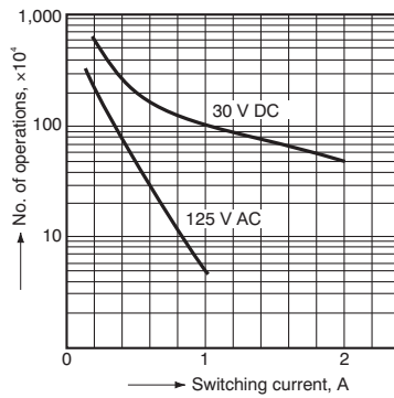
2. Life curve (Resistive load)
