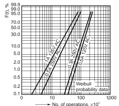
3. Contact reliability for AC loads
