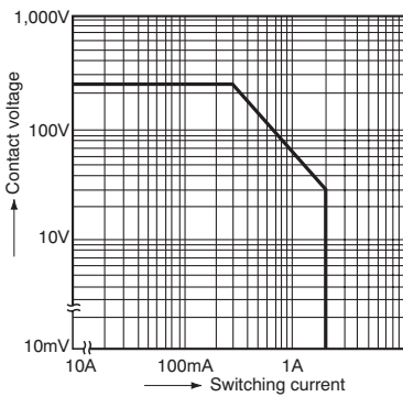
1. Maximum switching capacity
