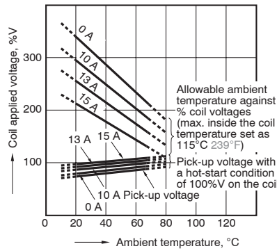
5.-(2) Ambient temperature characteristics (High capacity 15 A type, 1 Form A)
