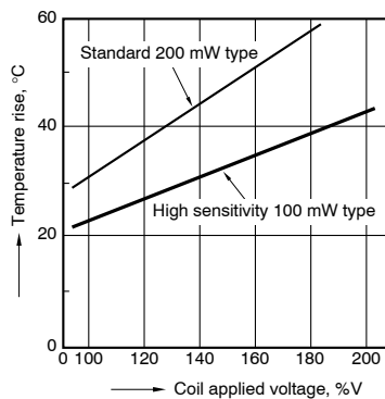
3.-(3) Coil temperature rise (High sensitivity type) Measured portion: Inside the coil
