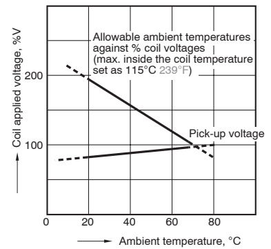
5.-(3) Ambient temperature characteristics (1 Form C type)
