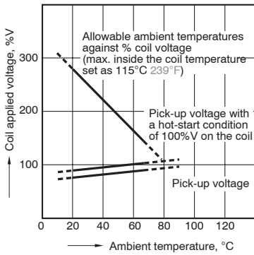
5.-(4) Ambient temperature characteristics (High sensitivity type)
