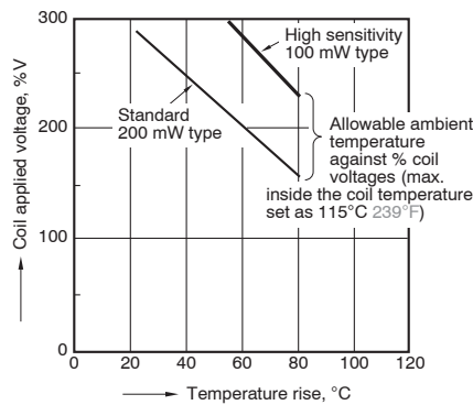
5.-(4) Ambient temperature characteristics (High sensitivity type)
