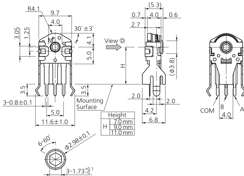
Shaft hole shape and dimension
