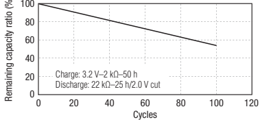
■ Charge/discharge cycle characteristics (Example: MS614)
