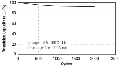
■ Charge/discharge cycle characteristics (Example: MT920)
