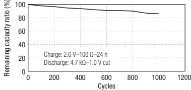
■ Charge/discharge cycle characteristics (Example: CTL920F)
